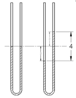
U-tube Manometer at 0 in. wg. The fluid is level U-tube Manometer at 4 in. wg. As measured from the top of each column of fluid (not from 0)
