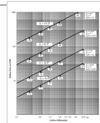
FIGURE 5-3 TYPICAL ORIFICE FLOW CURVES
