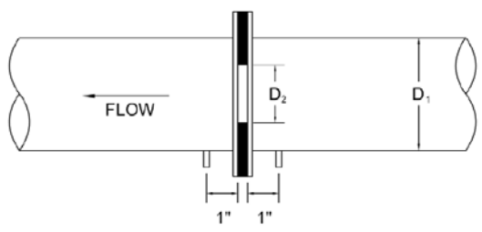
LOCATION OF FLANGE TAPS USE 3/32" OR 1/8" STEEL SQUARE EDGE ORIFICE PLATE
