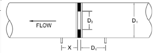
LOCATION OF VENA CONTRACTA TAPS USE 3/32" OR 1/8" STEEL SQUARE EDGE ORIFICE PLATE
