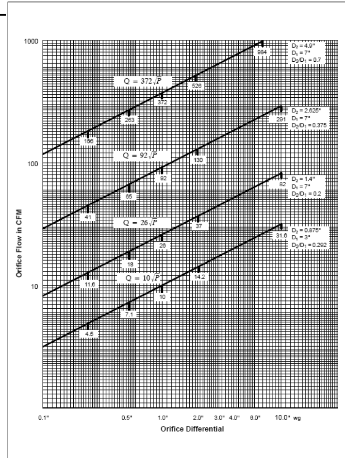
FIGURE 5-3 TYPICAL ORIFICE FLOW CURVES
