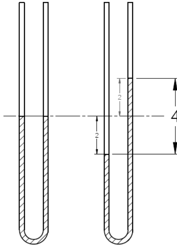
Utube Manometer at 0 in. w.g. The fluid is level
