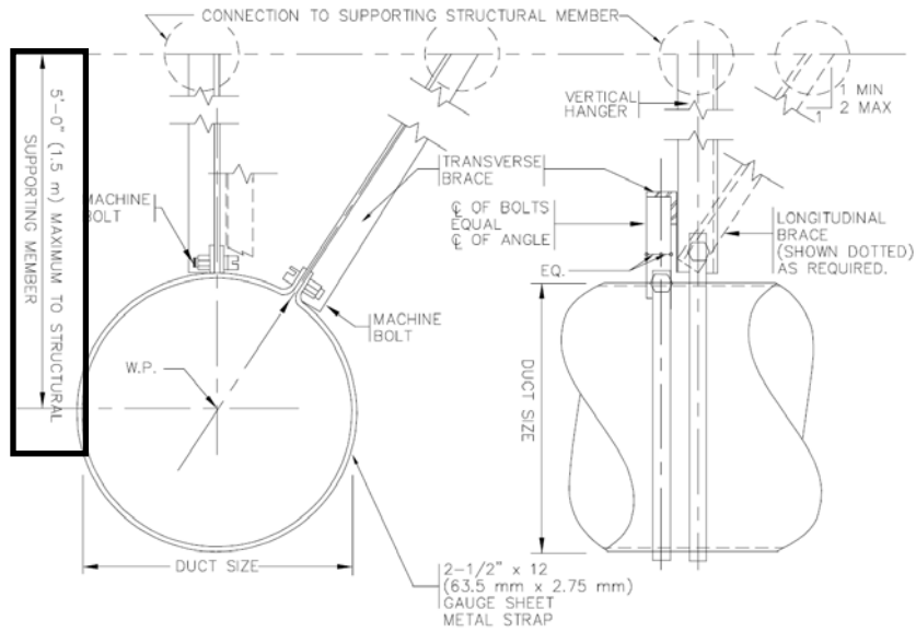
FIGURE 4-9 SINGLE HANGER SPACING FOR ROUND DUCTS 33-36 INCHES (838-900 MM)
