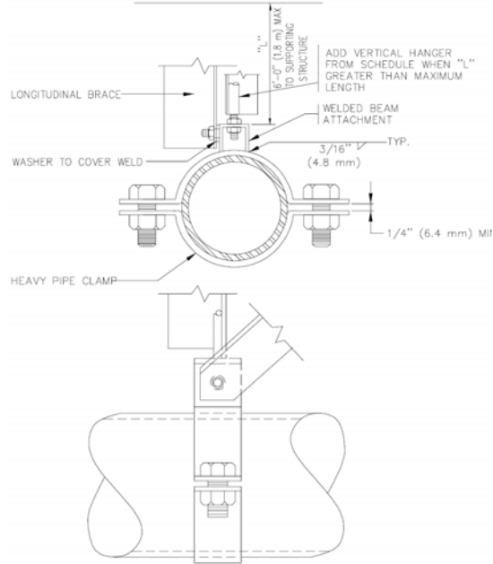
FIGURE 4-16 LONGITUDINAL BRACING FOR PIPES
