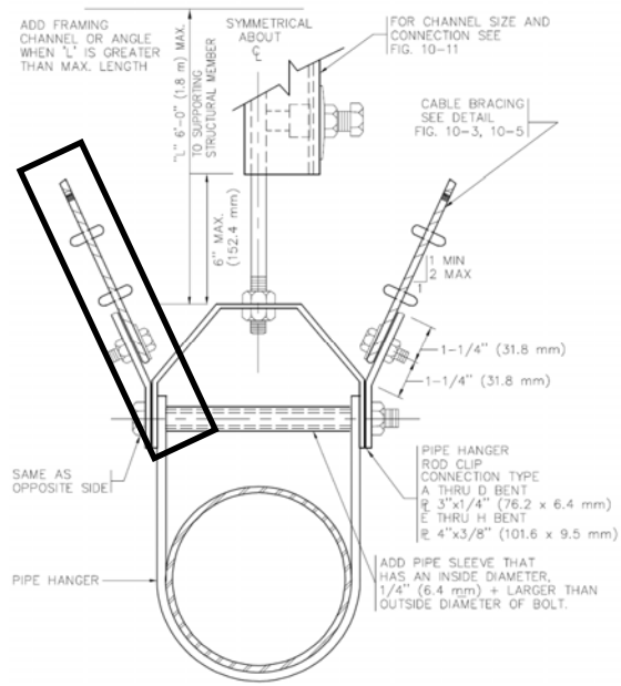
FIGURE 4-18 TRANSVERSE CABLE BRACING FOR PIPES
