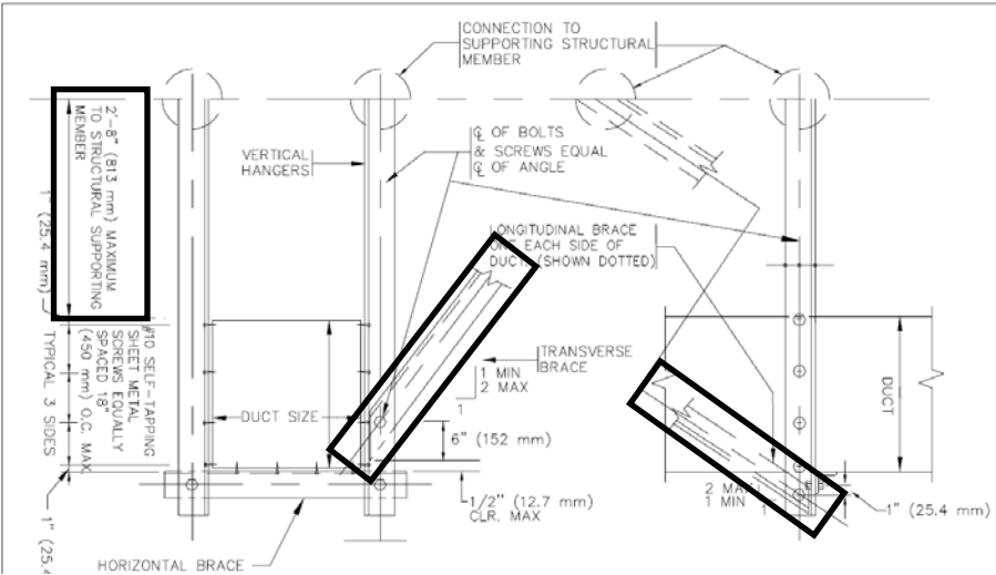
FIGURE 4-2 SIDE BRACING FOR RECTANGULAR DUCTS
