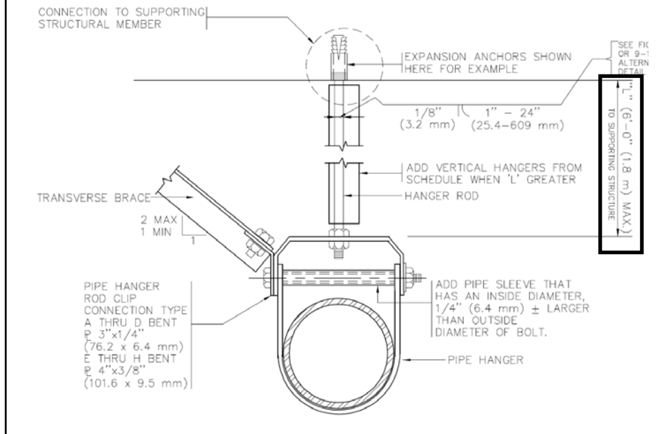
FIGURE 4-13 TRANSVERSE BRACING FOR PIPES
