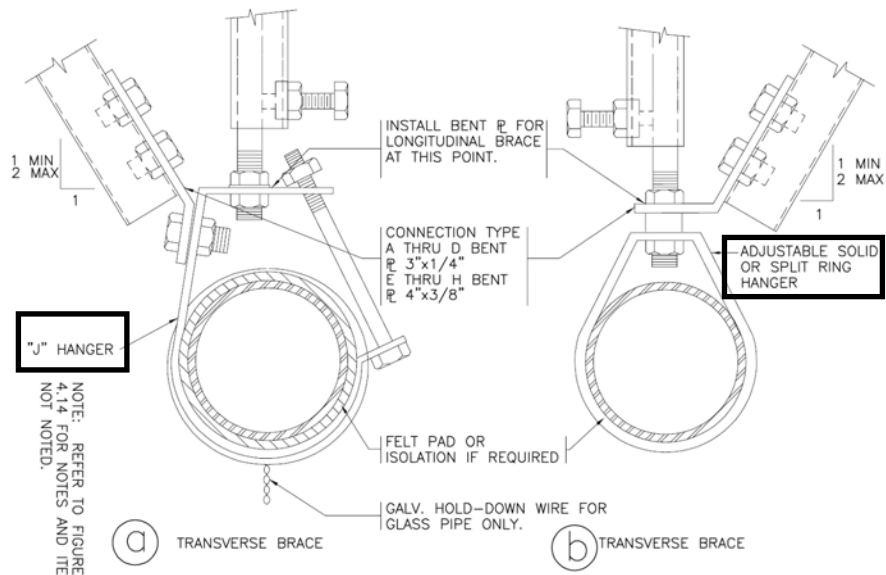
FIGURE 4-15 ALTERNATE ATTACHMENT TO HANGER FOR PIPE BRACING
