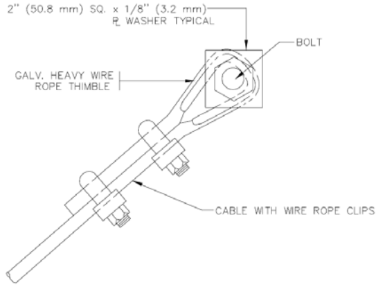
• Figure 10-5 Cable End Connections
