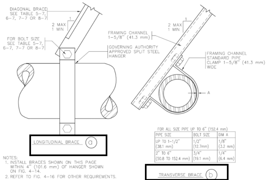
FIGURE 4-17 ALTERNATE BRACING FOR PIPES
