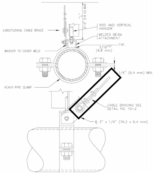
FIGURE 4-19 LONGITUDINAL CABLE BRACING FOR PIPES
