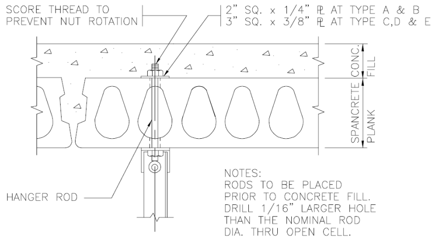
a CONNECTION TO HOLLOW CORE PLANK TYPE A, B, C, D, & E
