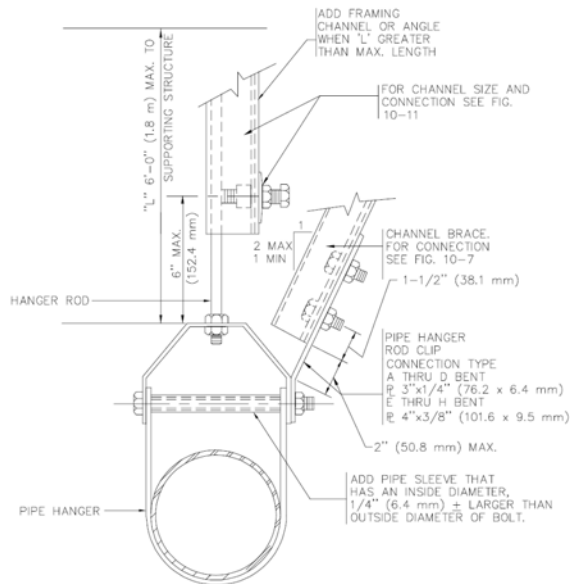
FIGURE 4-14 TRANSVERSE STRUT BRACING FOR PIPES
