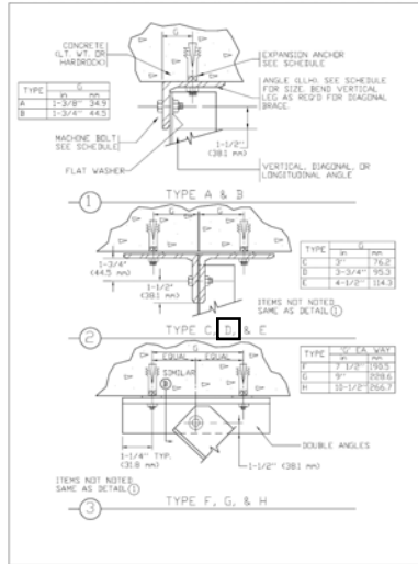
FIGURE 9-1 CONNECTIONS TO CONCRETE
